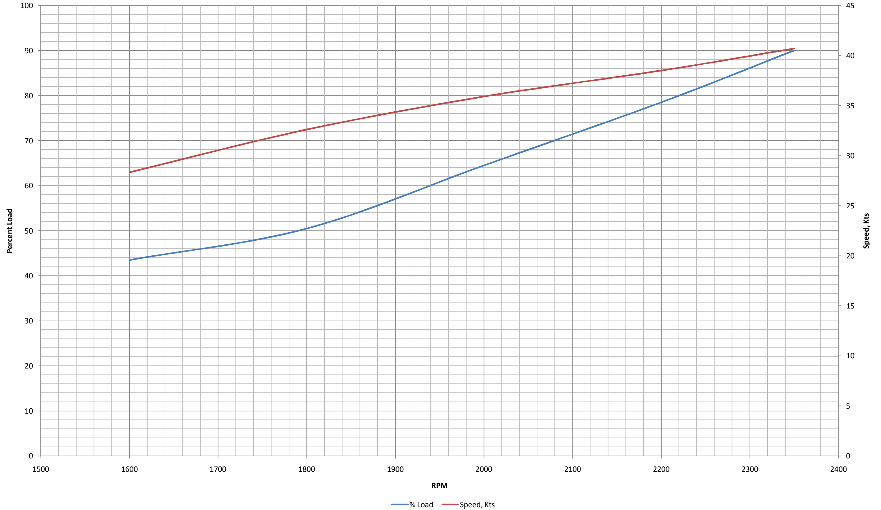
Speed and % Load vs RPM
